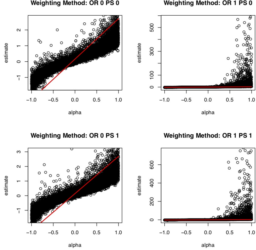
Figure 3.2: Sensitivity analysis results for the mean outcome estimation, weighting method. Results are shown for 10,000 simulated datasets with different values of \alpha . The target parameter is shown in red.
